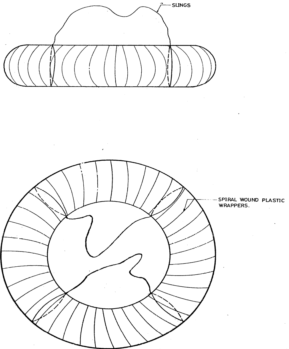
Fig. 1 - SLING ARRANGEMENT FOR LIFTING 63 mm \phi COILS
